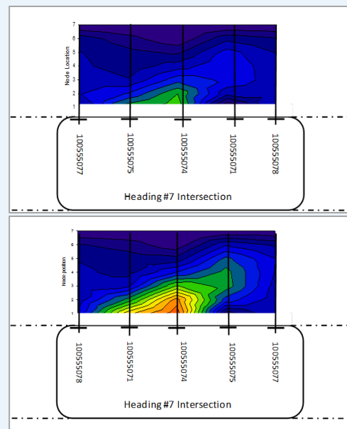
Fig 10: An array of 10 digi 6 Bolt with staggered gauges delineating an asymmetric fracture zone above an intersection ( max load is 1500 \epsilon\mu or 10tons)
