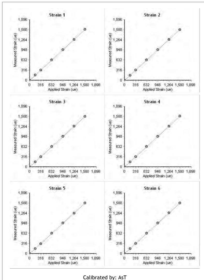
Fig. 4: Calibration sheet for a typical digi 6 -BOLT.
