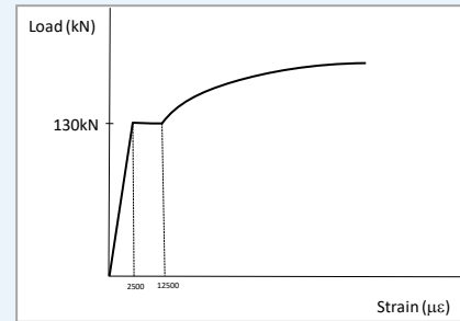
Fig.9. The load versus strain profile for a typical # 7 Bolt.
