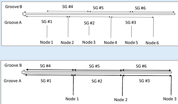
Fig 4. digi 6 Bolt Staggered (upper) and stacked (lower) strain gauge configurations. Gauges 1 and 4 are closest to the head.
